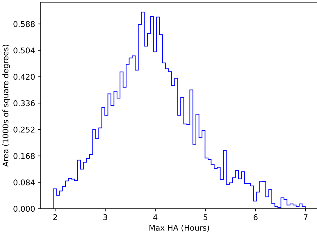
too_elab_r8_d3_giz_v3.4_10yrs WFD u band: Max HA
