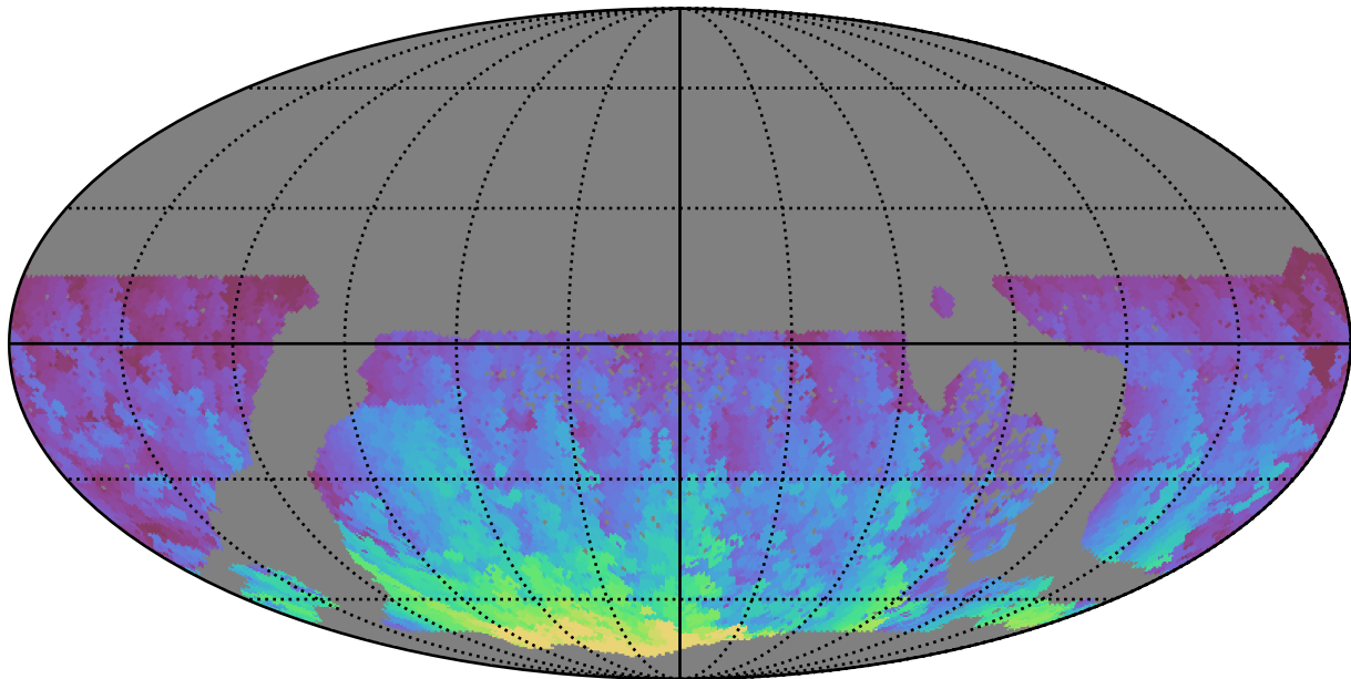
too_elab_r8_d3_giz_v3.4_10yrs WFD r band: Max HA
