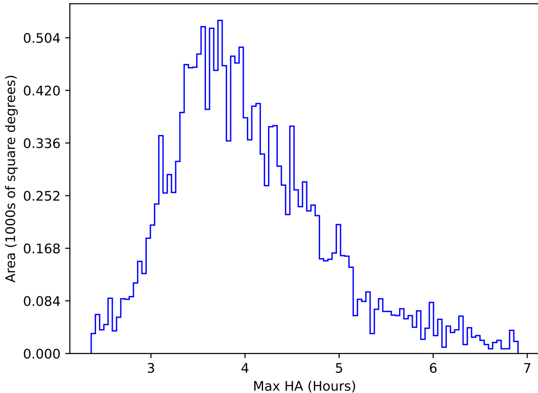
too_elab_r8_d3_giz_v3.4_10yrs WFD g band: Max HA
