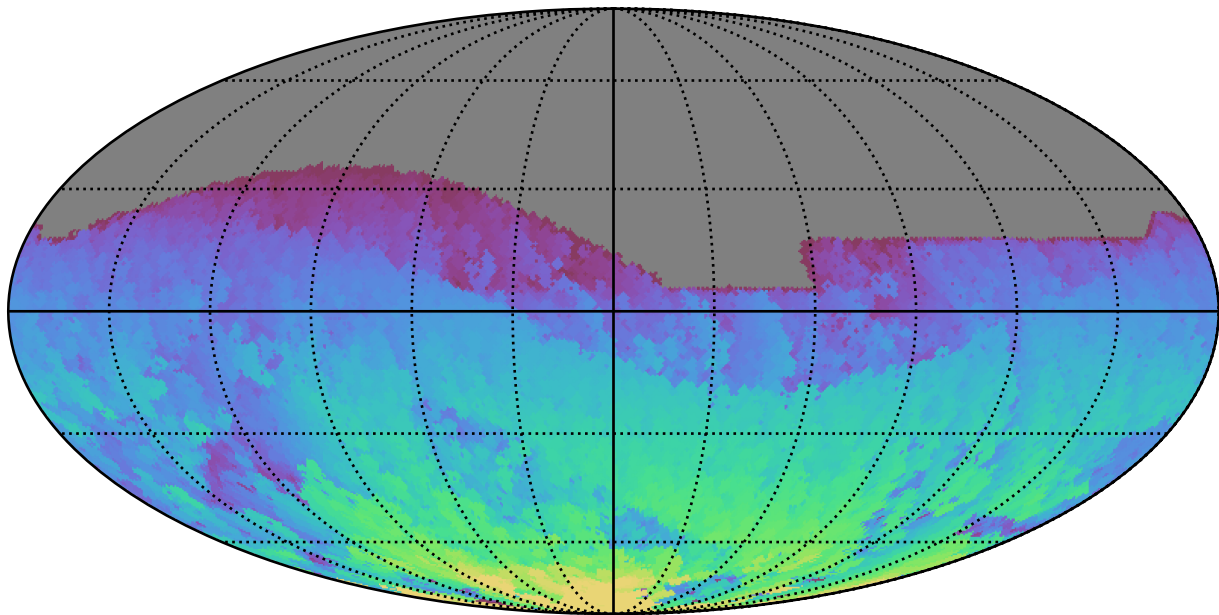
too_elab_r8_d3_giz_v3.4_10yrs All sky z band: Max HA
