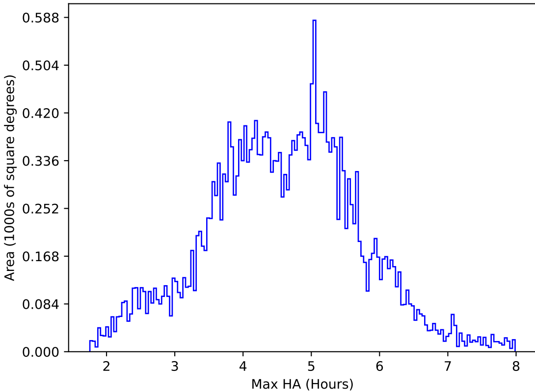
too_elab_r8_d3_giz_v3.4_10yrs All sky z band: Max HA
