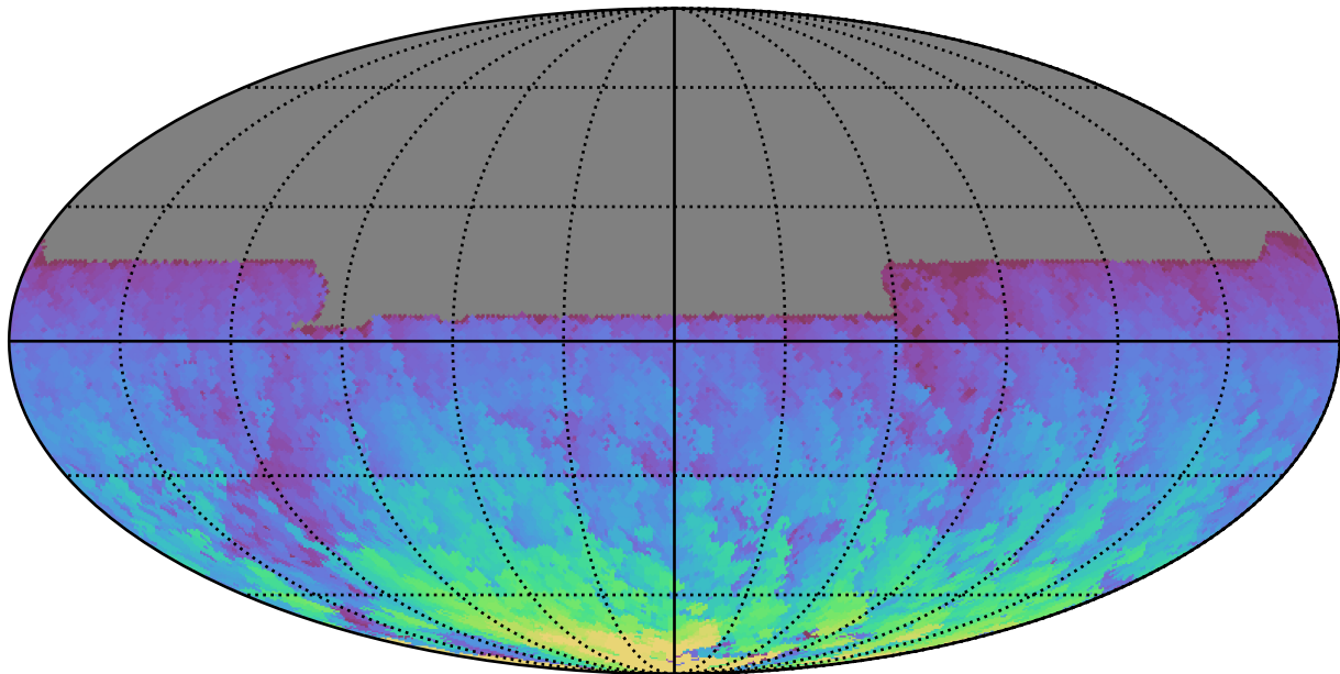
too_elab_r8_d3_giz_v3.4_10yrs All sky y band: Max HA
