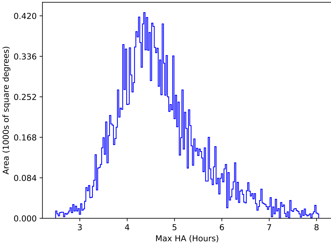
too_elab_r8_d3_giz_v3.4_10yrs All sky y band: Max HA
