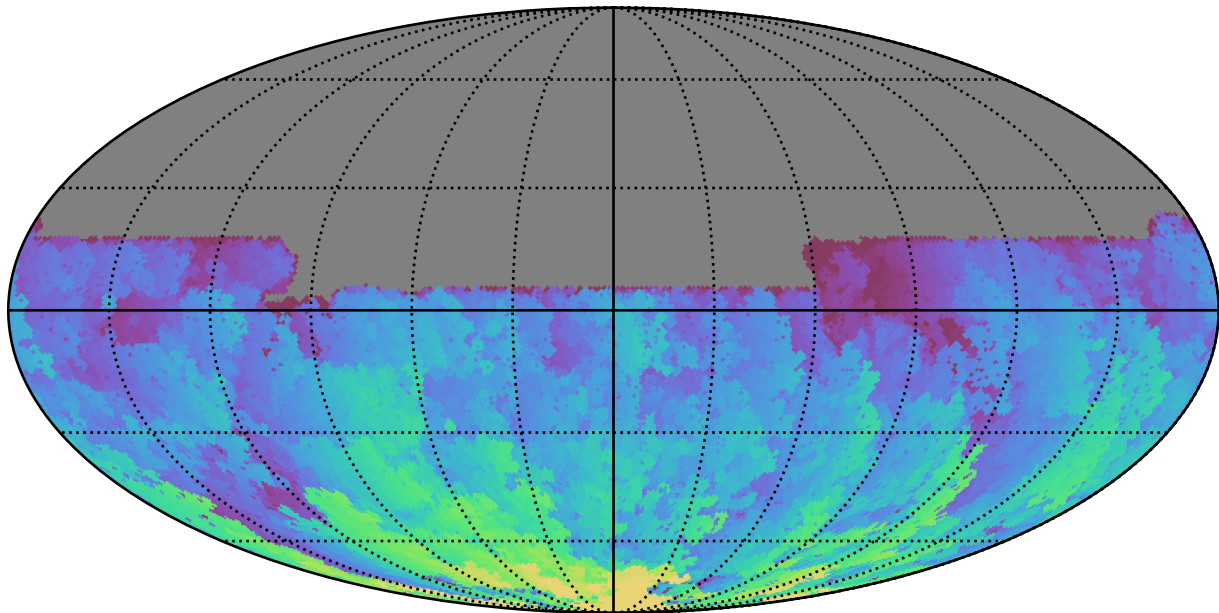
too_elab_r8_d3_giz_v3.4_10yrs All sky u band: Max HA
