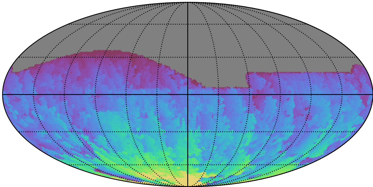
too_elab_r8_d3_giz_v3.4_10yrs All sky r band: Max HA
