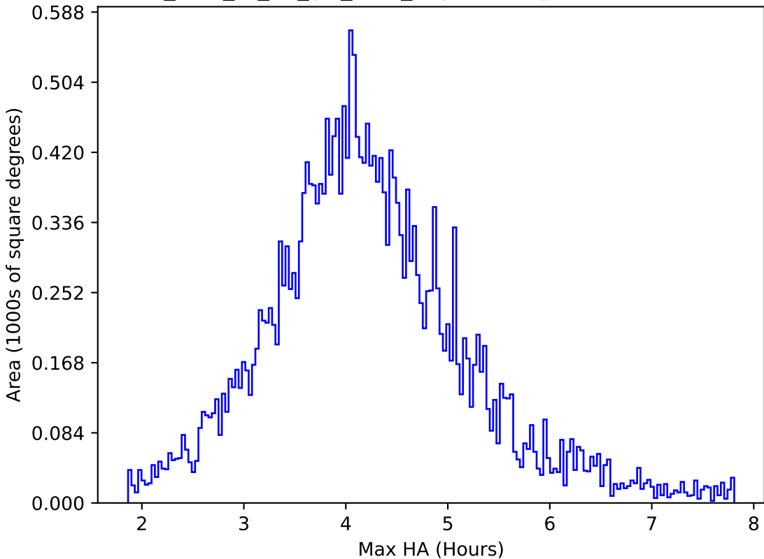
too_elab_r8_d3_giz_v3.4_10yrs All sky r band: Max HA
