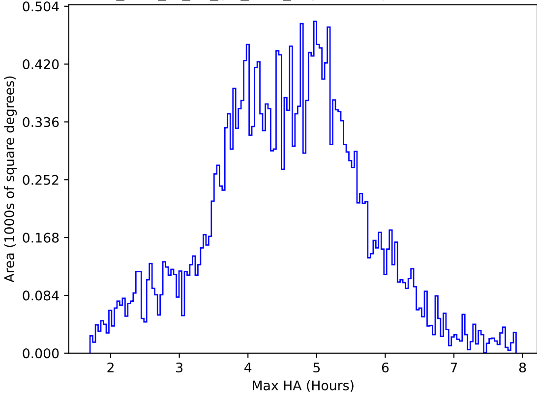
too_elab_r8_d3_giz_v3.4_10yrs All sky i band: Max HA
