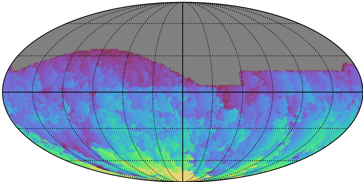
too_elab_r8_d3_giz_v3.4_10yrs All sky g band: Max HA
