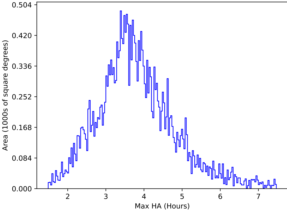
too_elab_r8_d3_giz_v3.4_10yrs All sky g band: Max HA
