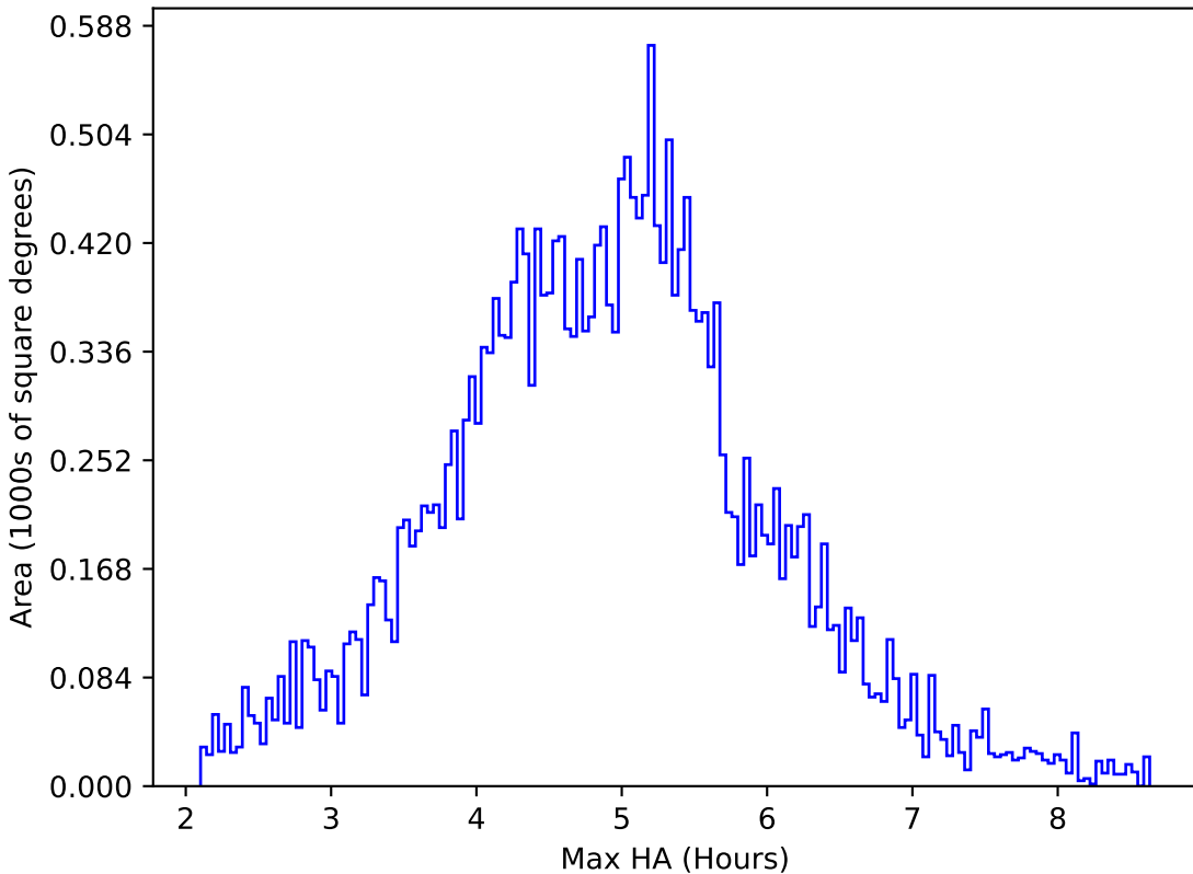
too_elab_r8_d3_giz_v3.4_10yrs All sky all bands: Max HA
