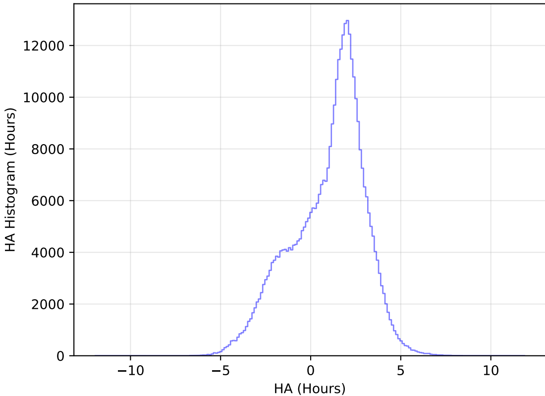
too_elab_r8_d3_giz_v3.4_10yrs WFD y band: HA Histogram
