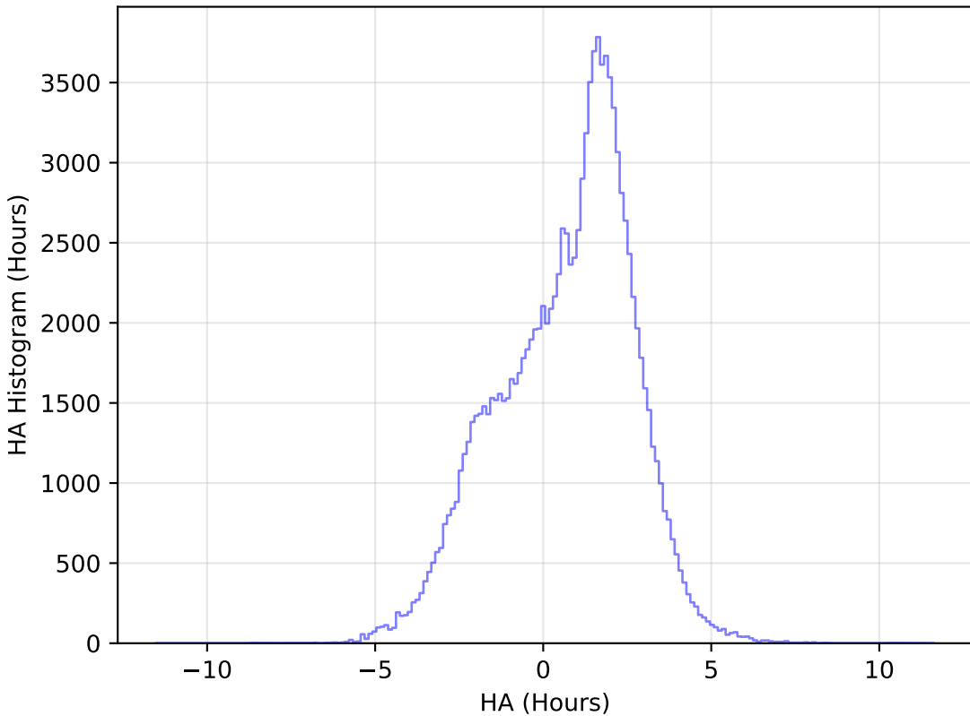
too_elab_r8_d3_giz_v3.4_10yrs WFD u band: HA Histogram
