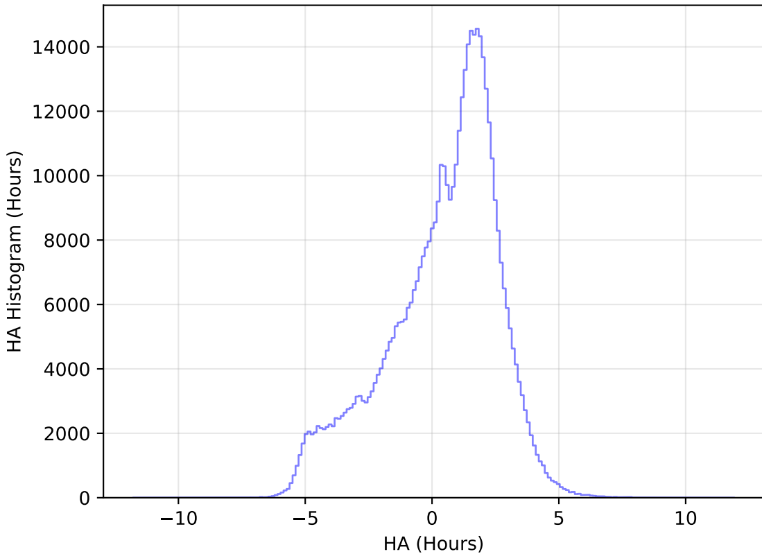
too_elab_r8_d3_giz_v3.4_10yrs WFD r band: HA Histogram
