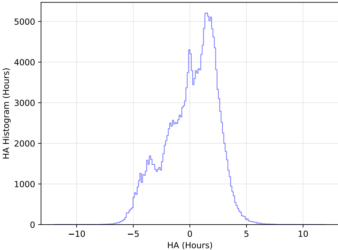
too_elab_r8_d3_giz_v3.4_10yrs WFD g band: HA Histogram
