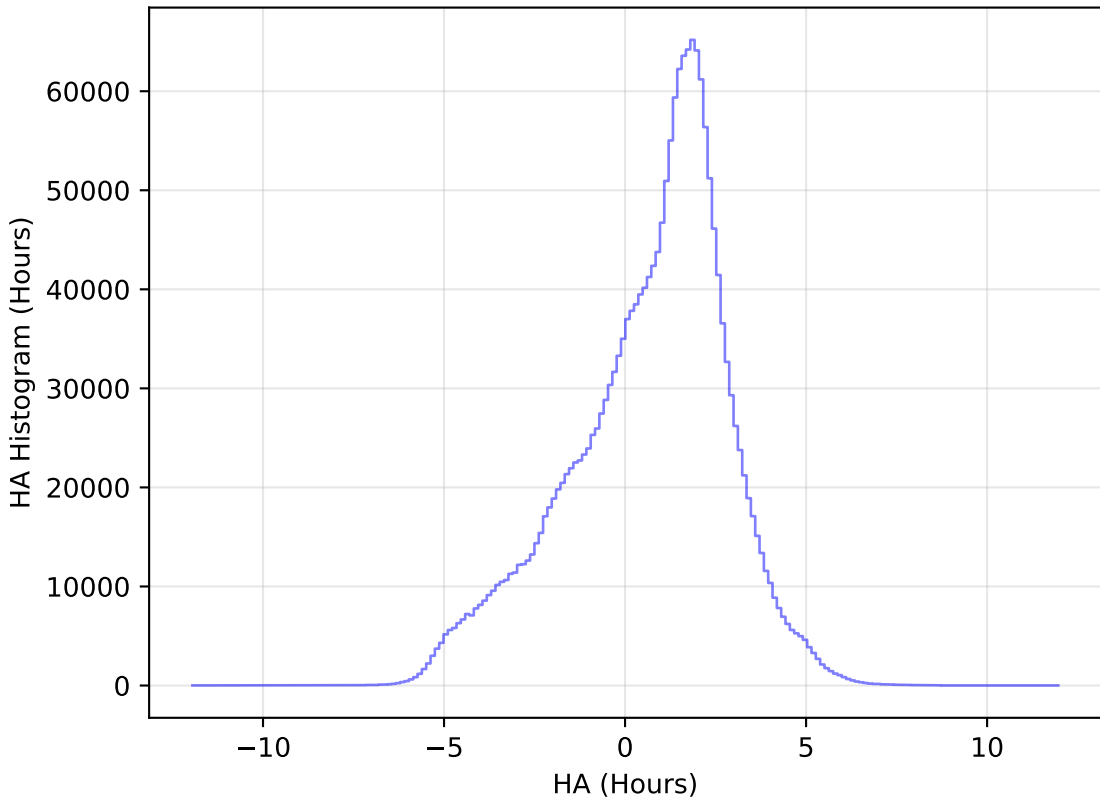
too_elab_r8_d3_giz_v3.4_10yrs WFD all bands: HA Histogram
