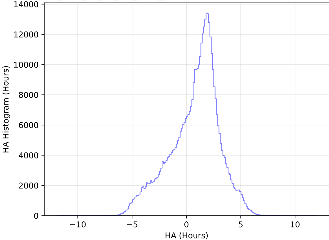
too_elab_r8_d3_giz_v3.4_10yrs All sky z band: HA Histogram
