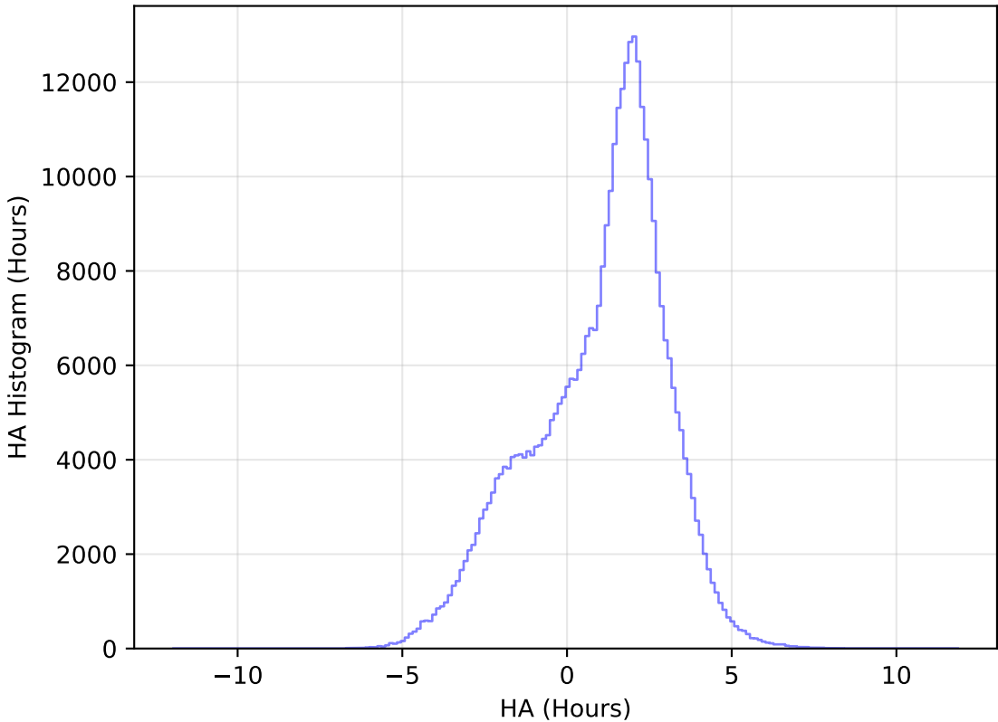
too_elab_r8_d3_giz_v3.4_10yrs All sky y band: HA Histogram
