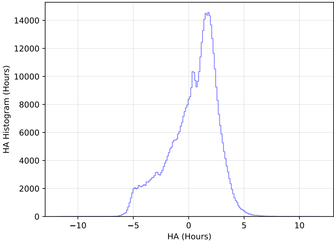
too_elab_r8_d3_giz_v3.4_10yrs All sky r band: HA Histogram
