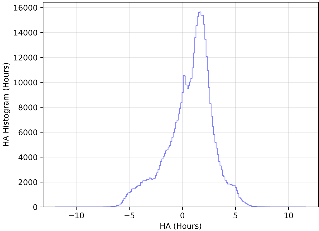
too_elab_r8_d3_giz_v3.4_10yrs All sky i band: HA Histogram
