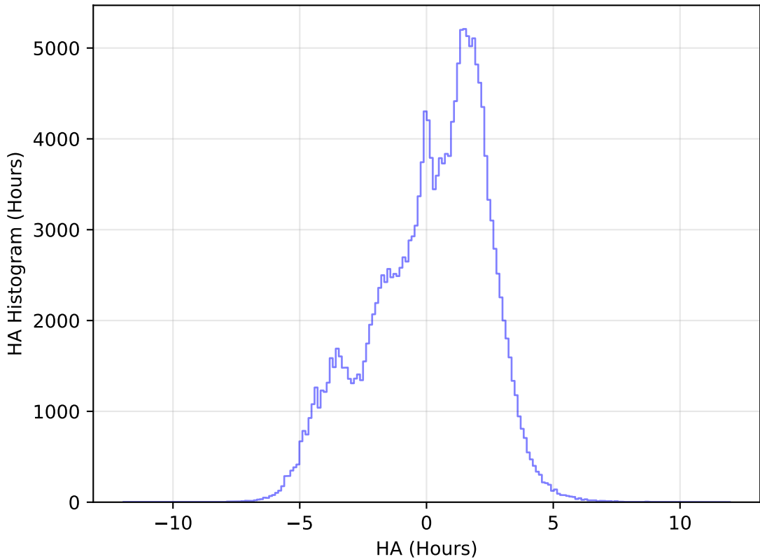
too_elab_r8_d3_giz_v3.4_10yrs All sky g band: HA Histogram
