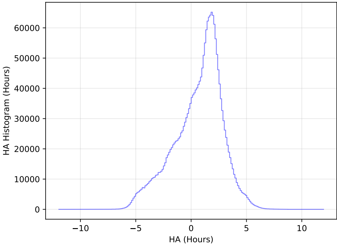
too_elab_r8_d3_giz_v3.4_10yrs All sky all bands: HA Histogram
