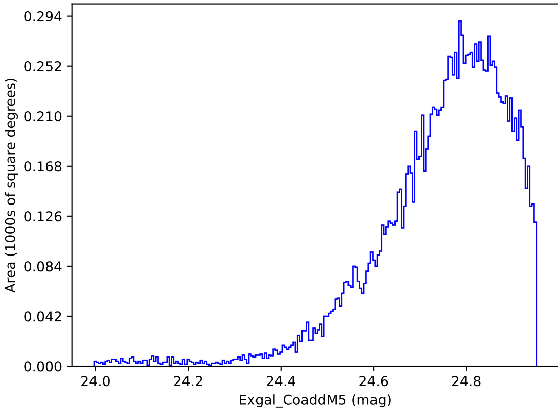
too_elab_r8_d3_giz_v3.4_10yrs WFD y band: Exgal_CoaddM5
