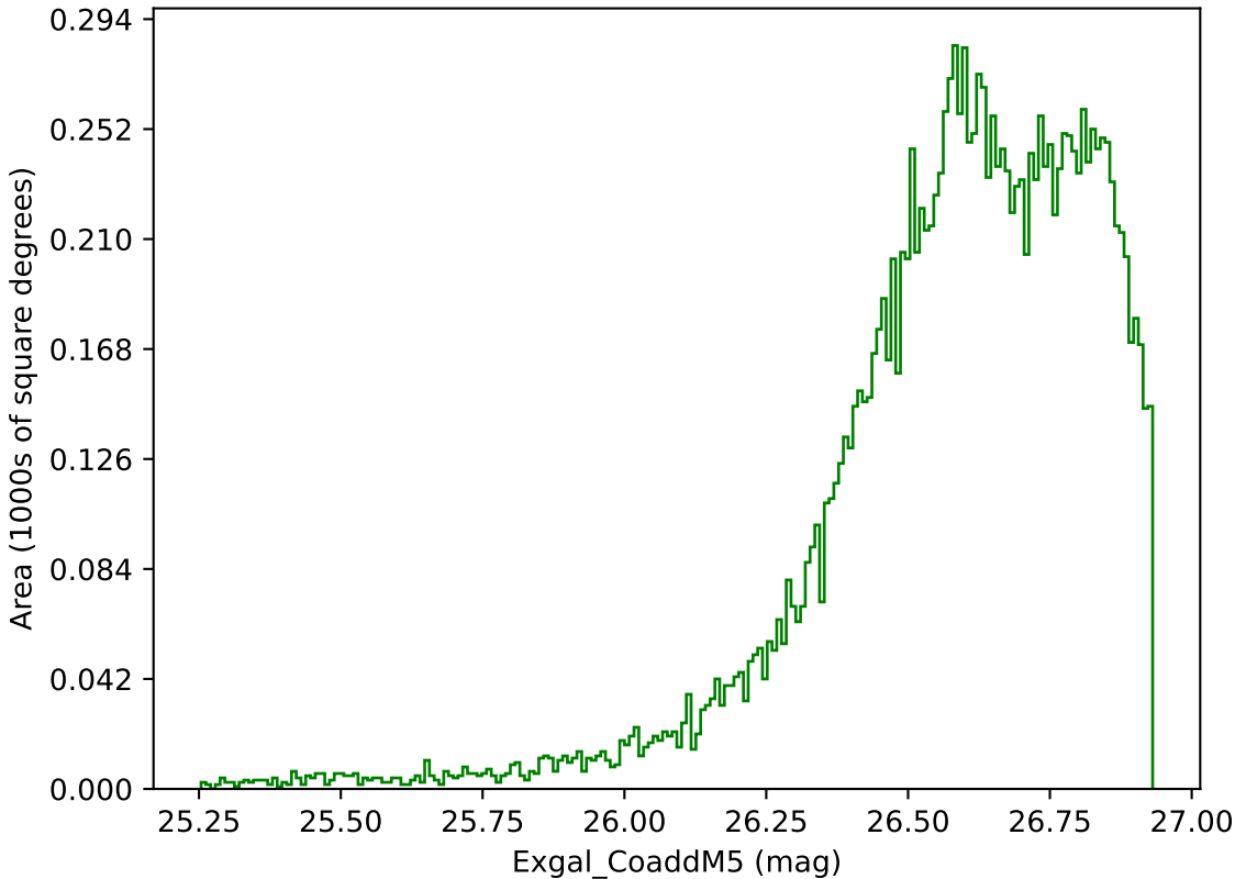
too_elab_r8_d3_giz_v3.4_10yrs WFD g band: Exgal_CoaddM5
