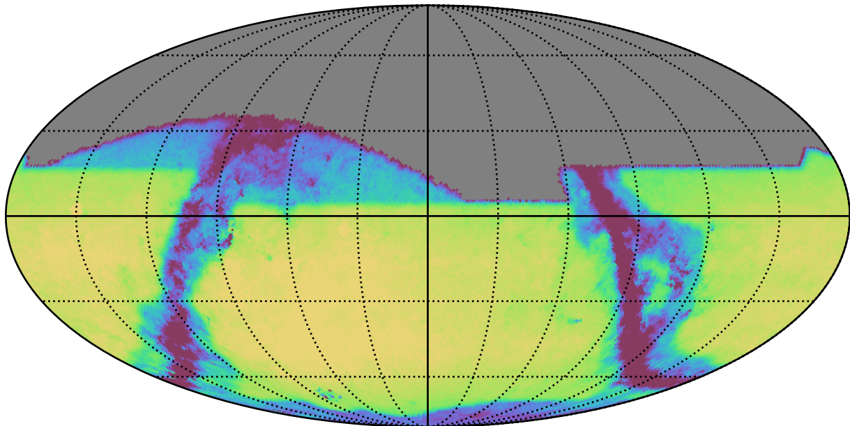
too_elab_r8_d3_giz_v3.4_10yrs All sky z band: Exgal_CoaddM5
