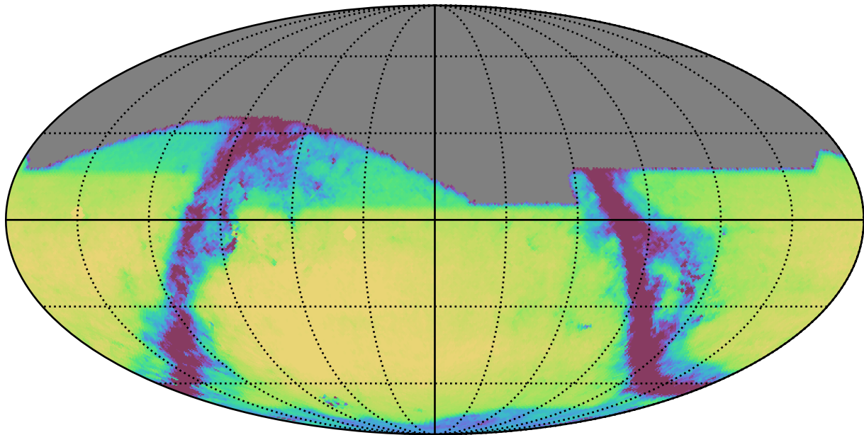
too_elab_r8_d3_giz_v3.4_10yrs All sky r band: Exgal_CoaddM5
