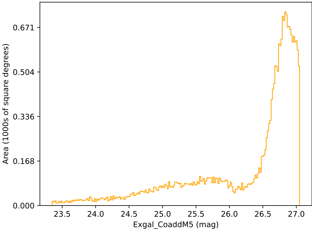
too_elab_r8_d3_giz_v3.4_10yrs All sky r band: Exgal_CoaddM5
