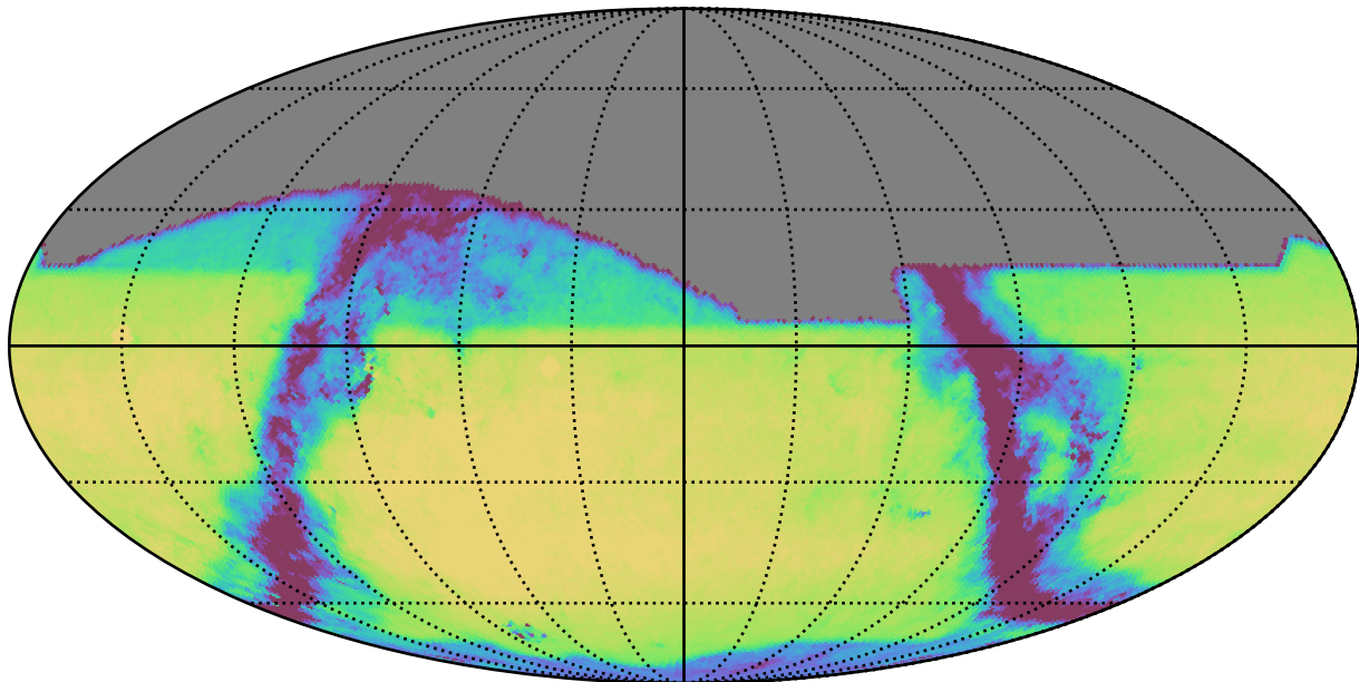
too_elab_r8_d3_giz_v3.4_10yrs All sky i band: Exgal_CoaddM5
