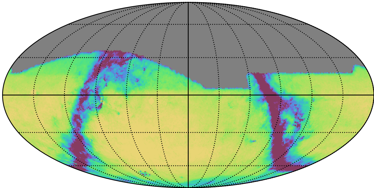
too_elab_r8_d3_giz_v3.4_10yrs All sky g band: Exgal_CoaddM5
