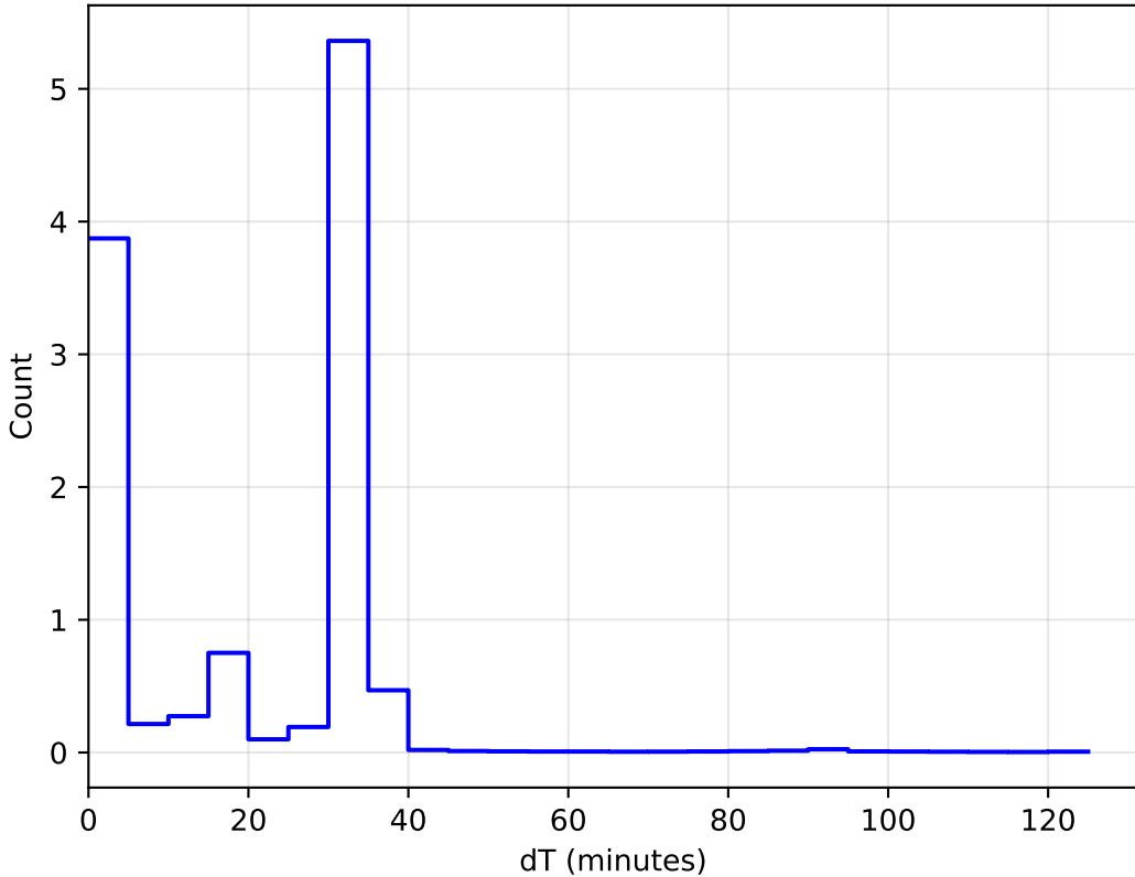
too_elab_r8_d3_giz_v3.4_10yrs WFD: DeltaT Histogram
