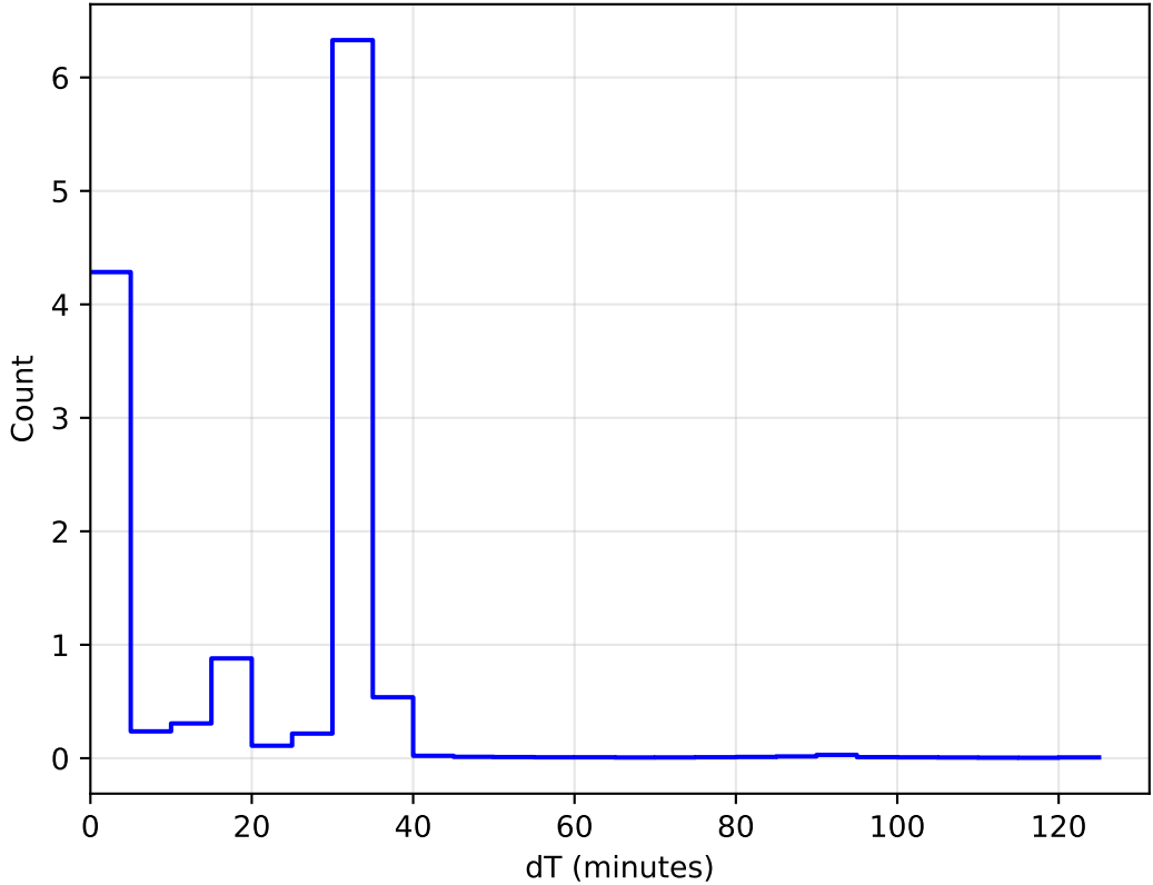
too_elab_r8_d3_giz_v3.4_10yrs All sky: DeltaT Histogram
