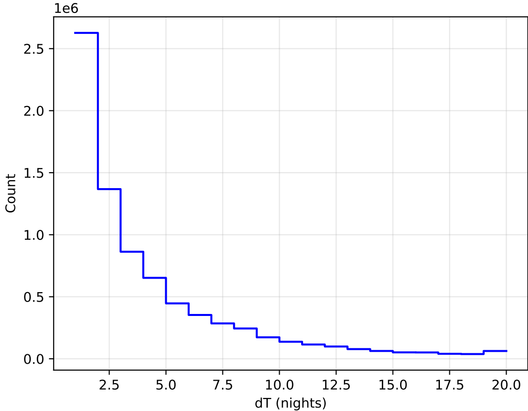
too_elab_r8_d3_giz_v3.4_10yrs WFD all bands: DeltaNight Histogram
