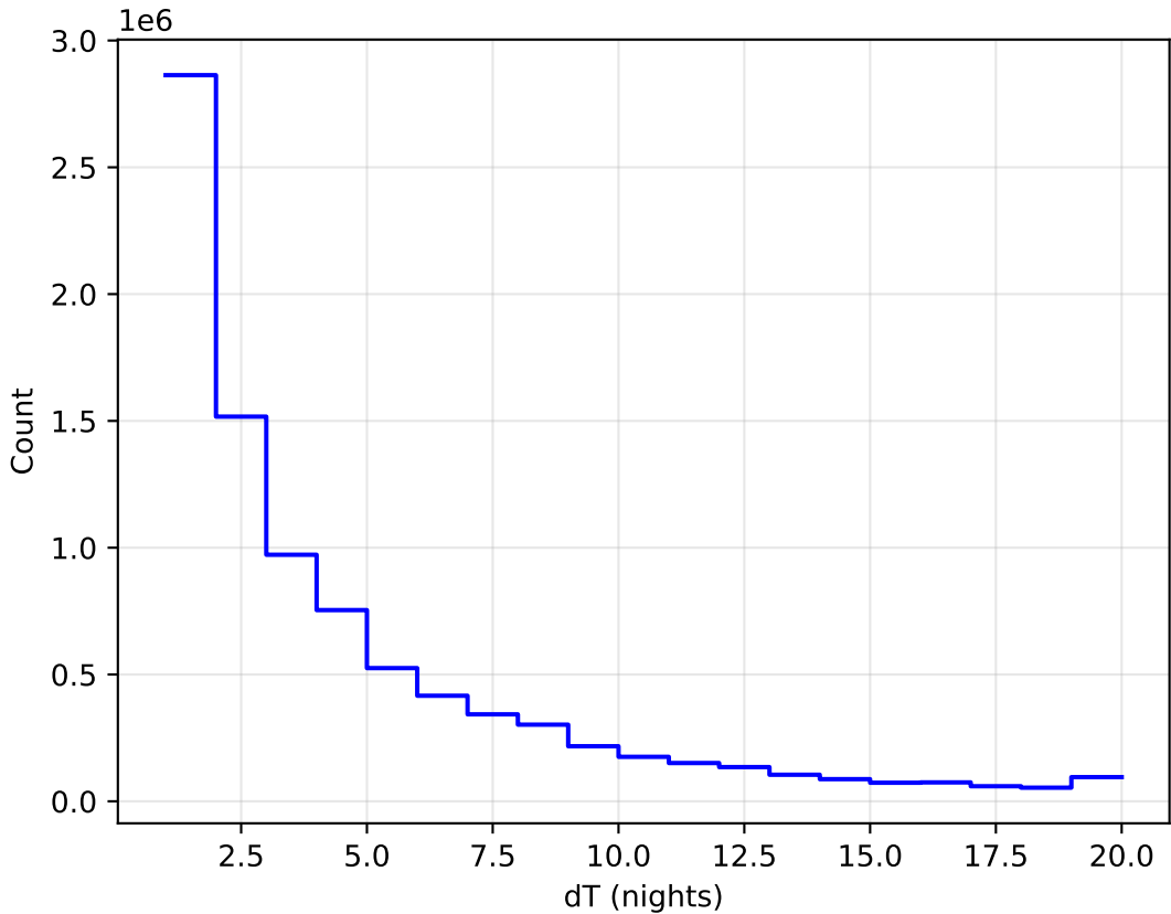
too_elab_r8_d3_giz_v3.4_10yrs All sky all bands: DeltaNight Histogram
