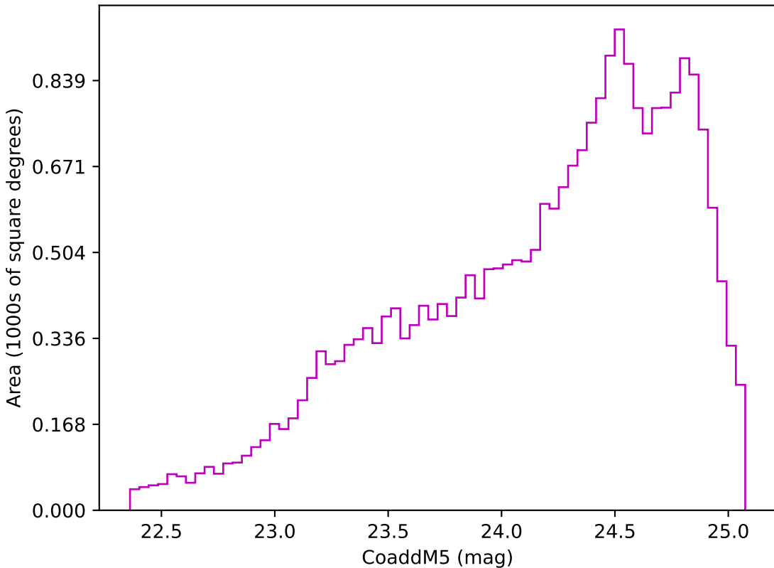
too_elab_r8_d3_giz_v3.4_10yrs Yr 3-4 z band: CoaddM5
