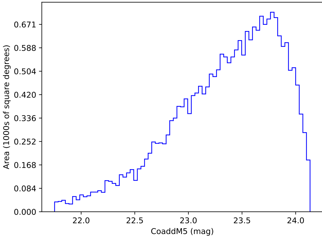
too_elab_r8_d3_giz_v3.4_10yrs Yr 3-4 y band: CoaddM5
