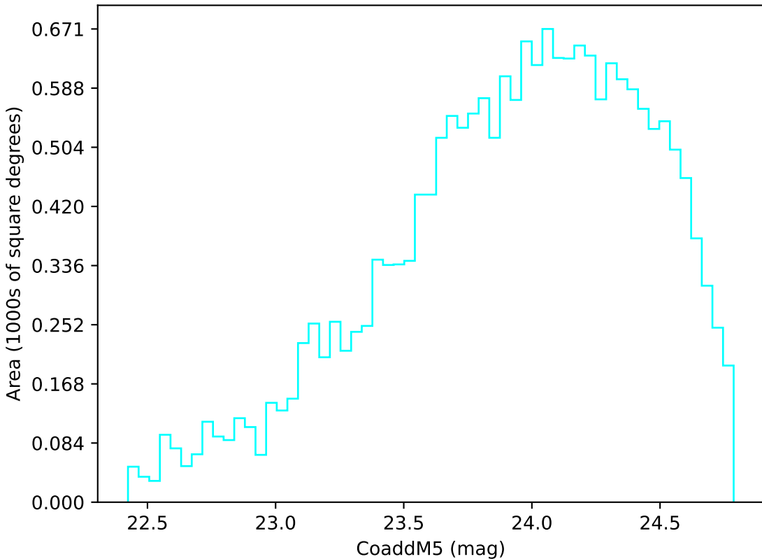
too_elab_r8_d3_giz_v3.4_10yrs Yr 3-4 u band: CoaddM5
