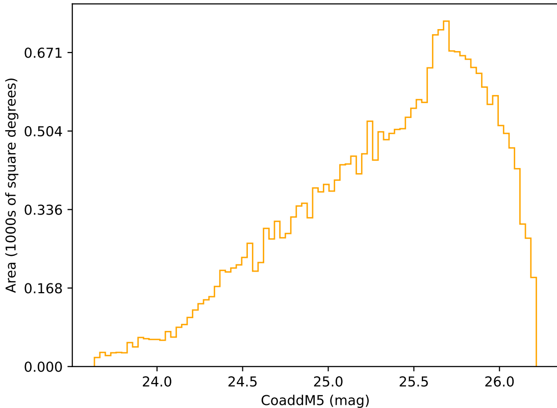
too_elab_r8_d3_giz_v3.4_10yrs Yr 3-4 r band: CoaddM5
