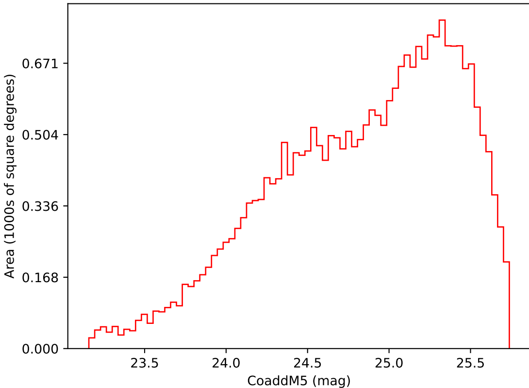
too_elab_r8_d3_giz_v3.4_10yrs Yr 3-4 i band: CoaddM5
