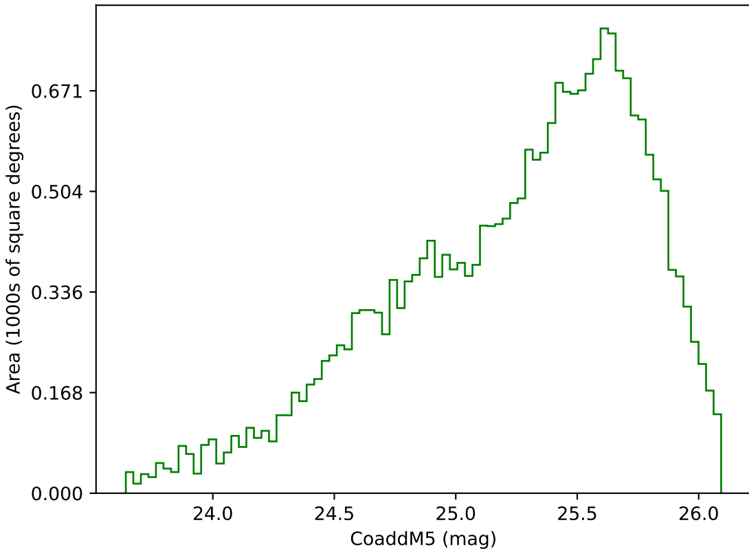
too_elab_r8_d3_giz_v3.4_10yrs Yr 3-4 g band: CoaddM5
