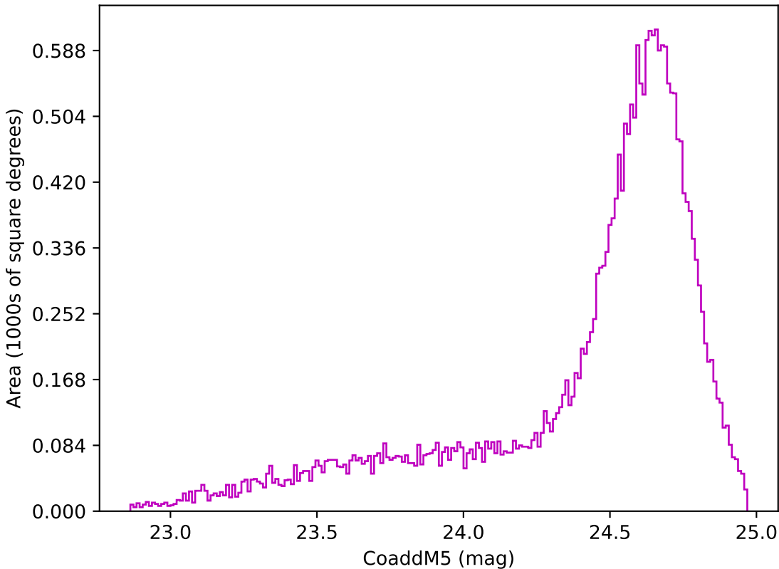
too_elab_r8_d3_giz_v3.4_10yrs Yr 1 z band: CoaddM5
