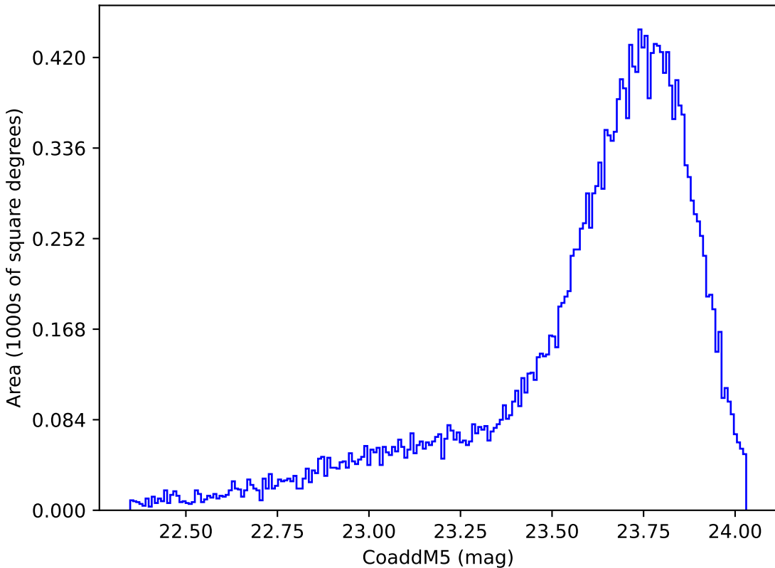
too_elab_r8_d3_giz_v3.4_10yrs Yr 1 y band: CoaddM5
