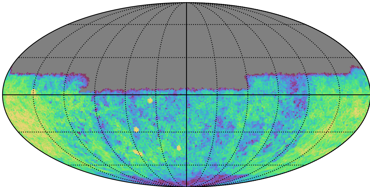
too_elab_r8_d3_giz_v3.4_10yrs Yr 1 u band: CoaddM5
