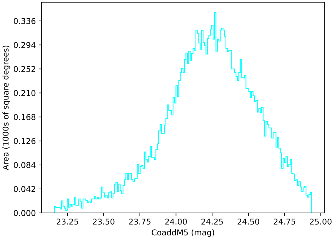
too_elab_r8_d3_giz_v3.4_10yrs Yr 1 u band: CoaddM5
