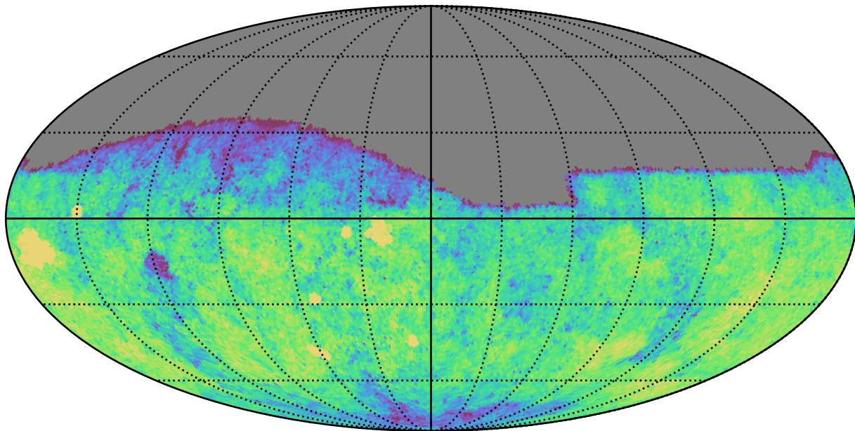
too_elab_r8_d3_giz_v3.4_10yrs Yr 1 g band: CoaddM5
