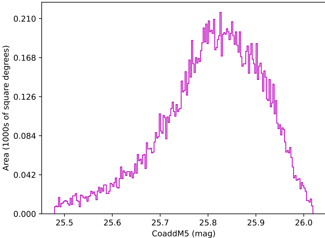
too_elab_r8_d3_giz_v3.4_10yrs WFD z band: CoaddM5
