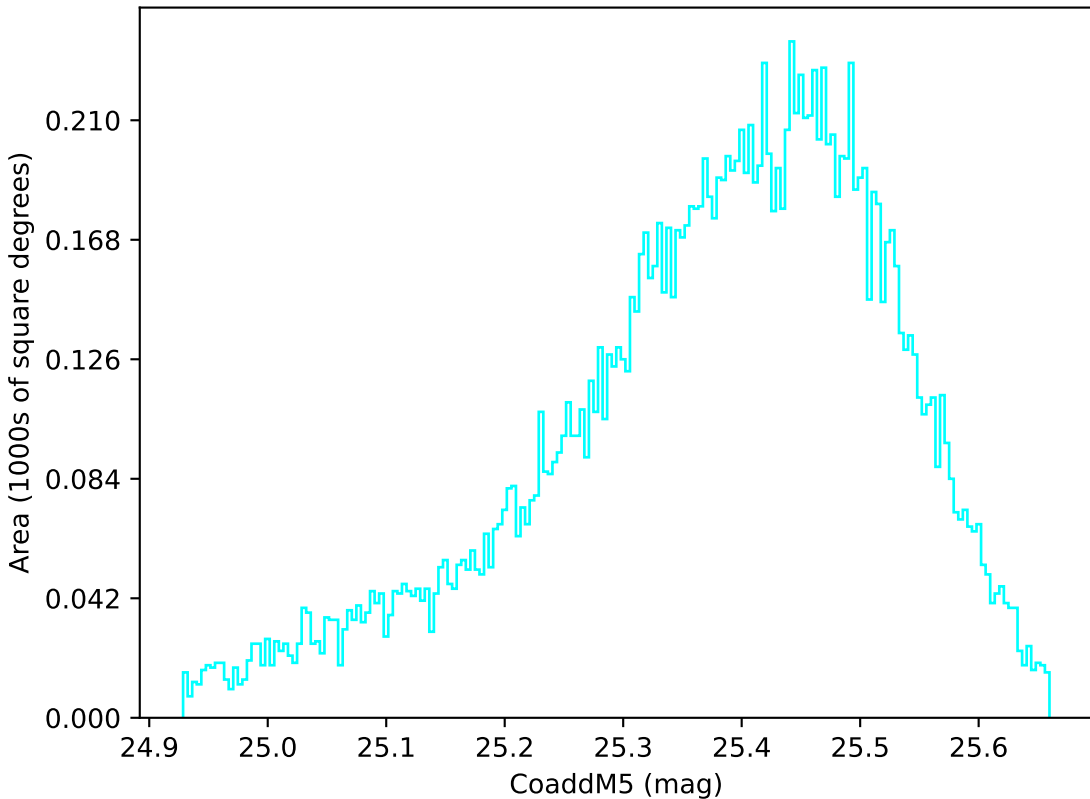
too_elab_r8_d3_giz_v3.4_10yrs WFD u band: CoaddM5
