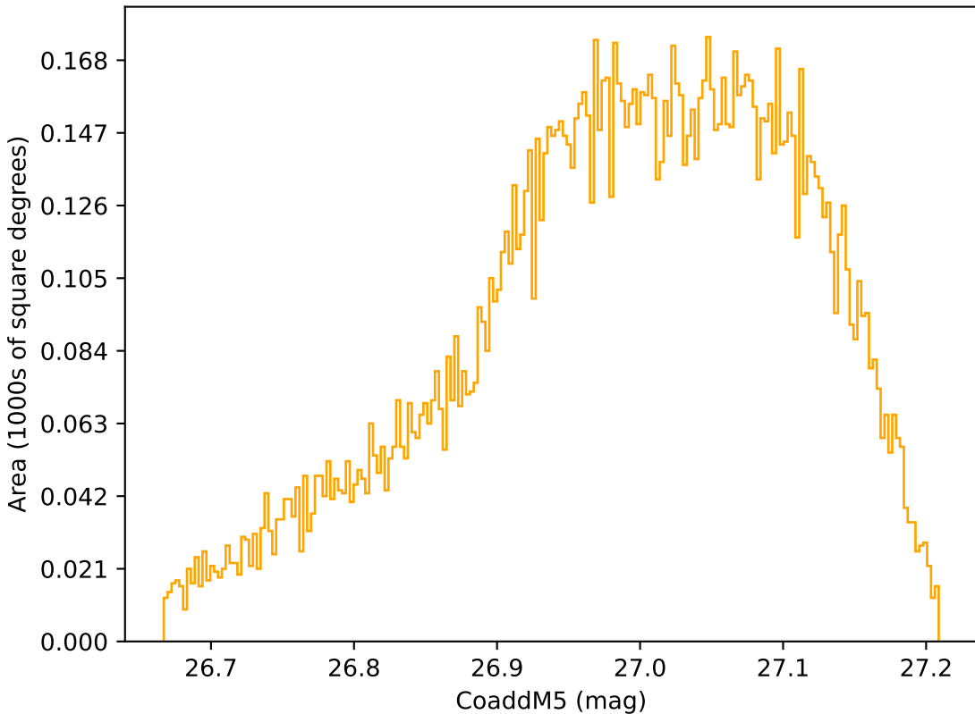
too_elab_r8_d3_giz_v3.4_10yrs WFD r band: CoaddM5
